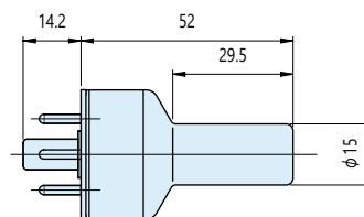
TG-550C Dimensions Diagram
